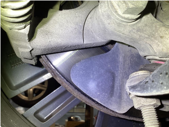
1.1 Slitte/stor slitekant
