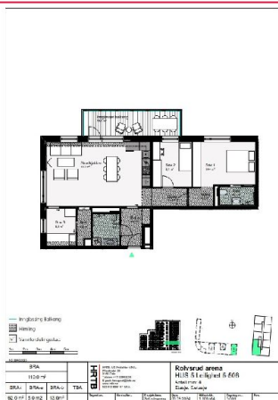
Plantegning 5-506
