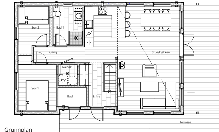
Grunnplan
