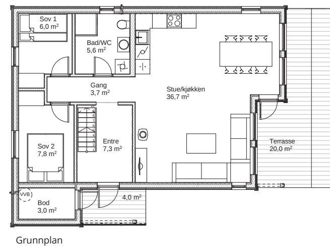
Grunnplan
