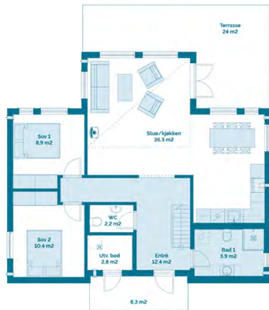
Grunnplan
