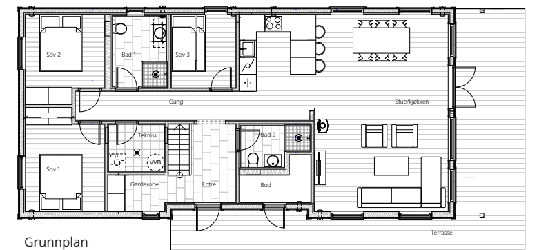
Grunnplan
