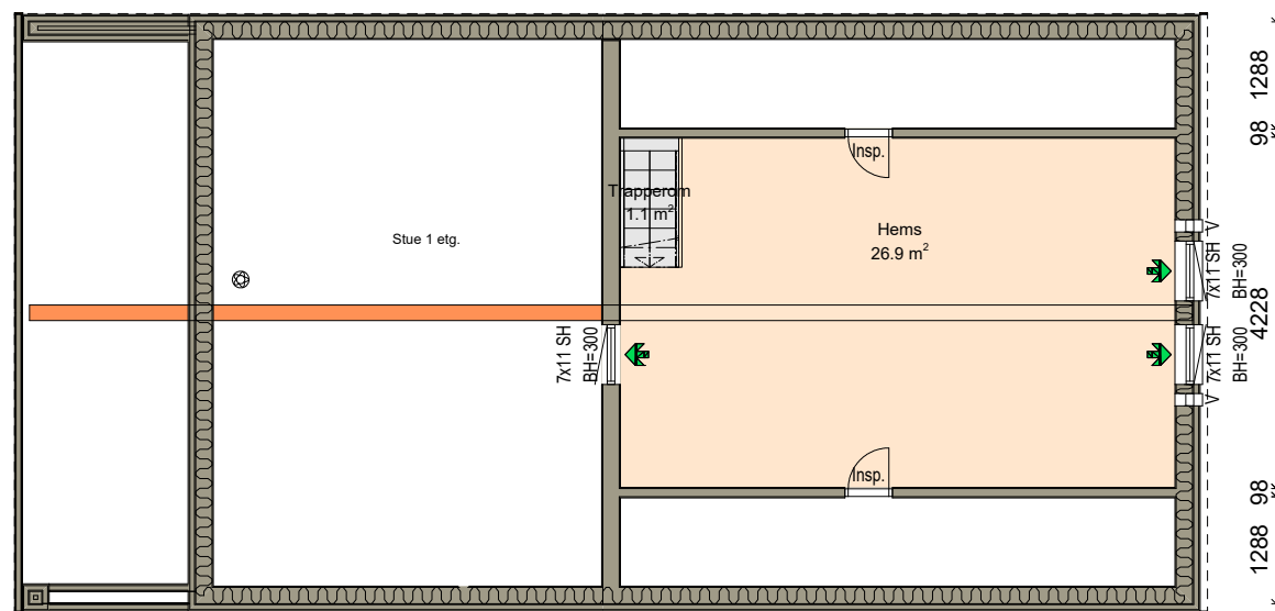
Plan hems
