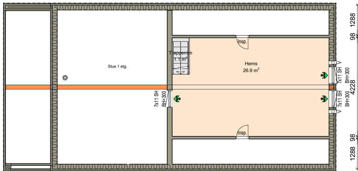
Plan hems
