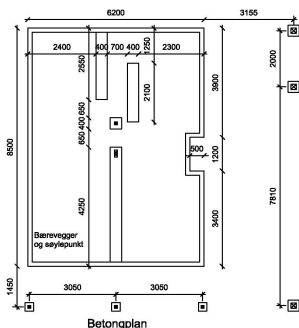
Betongplan
