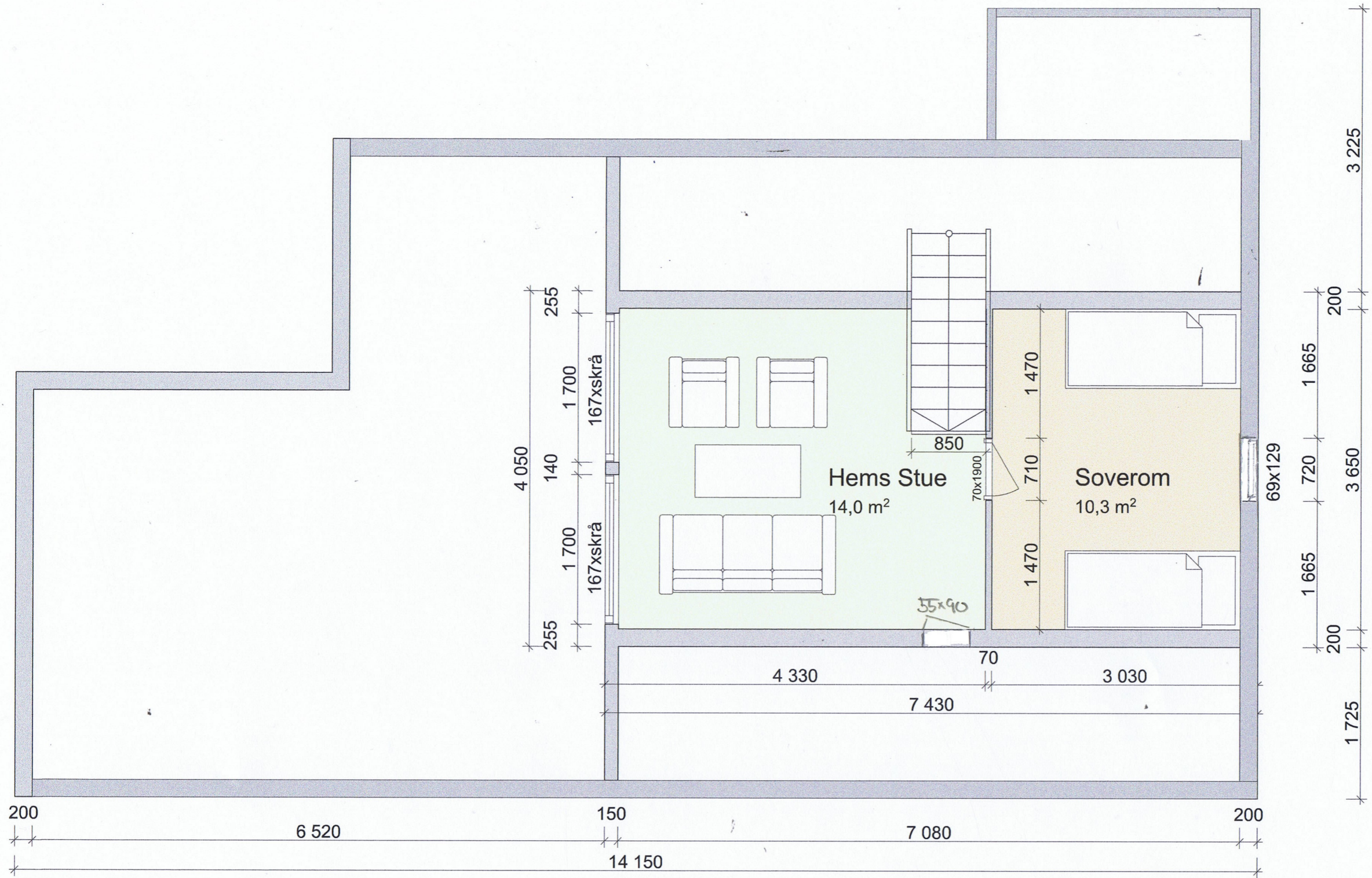
Hems plan
