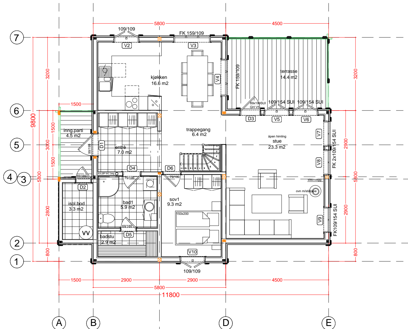
Plan 1 etg
