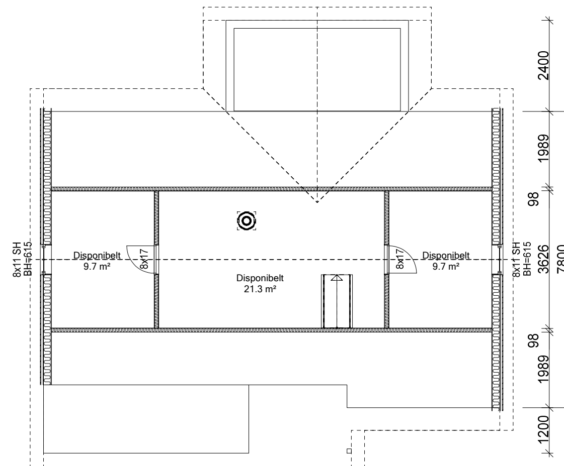
Plan hems
