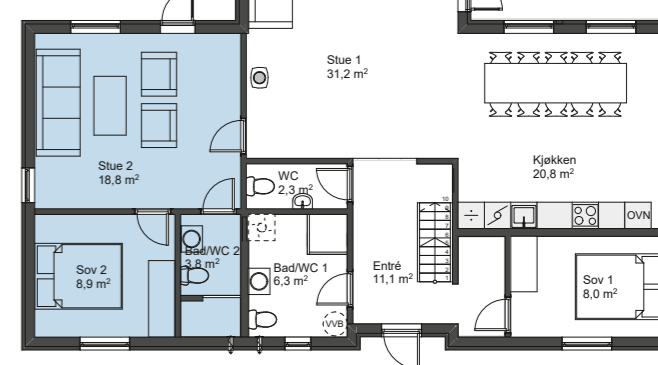
Grunnplan
