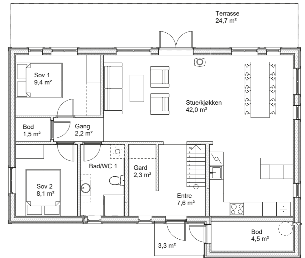
Grunnplan
