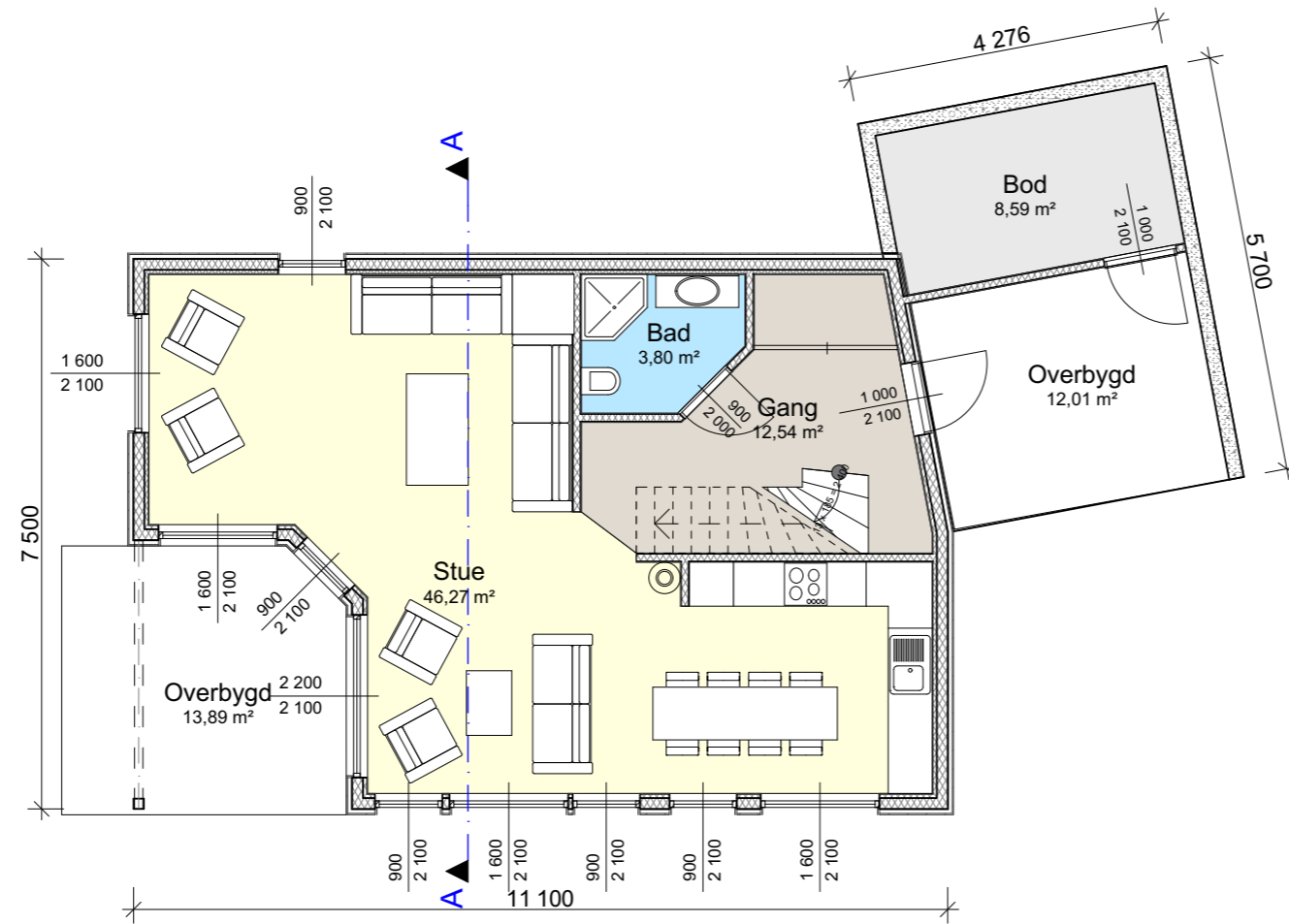
Plan 1 Etg
